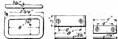
Figs. 5072-73. BOLSTER-HANGER AND U-BOLT.
